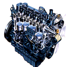
KUBOTA Diesel engine
