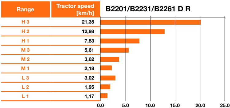
Speed diagram
